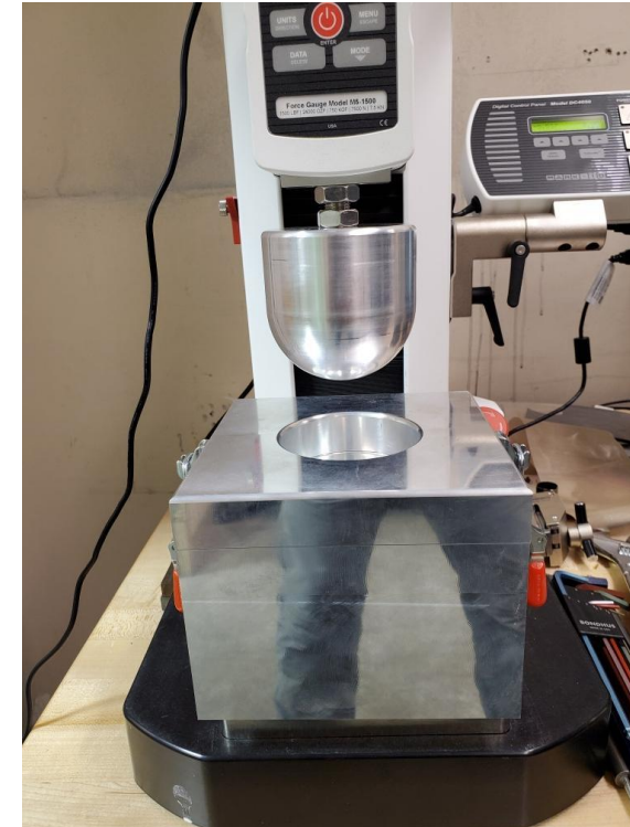
Dome/Erichsen-style fixture
