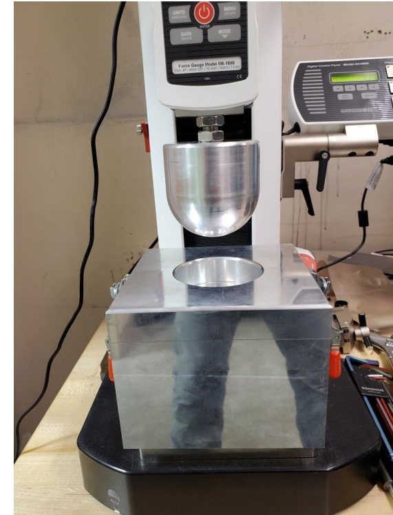
Dome/Ericksen-style fixture
