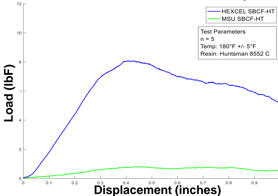
MSU SBCF vs. Hexcel SBCF: load vs. displacement
