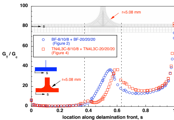
Fig. 10. Computed failure index - results for radius r=5.08 mm versus reference solution
