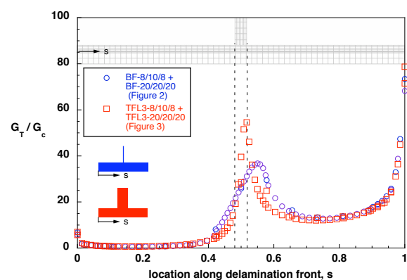
Fig. 6. Computed failure index – 3D web results versus reference solution
