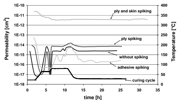
Fig. 10 Summary of the through thickness air permeability measurements
