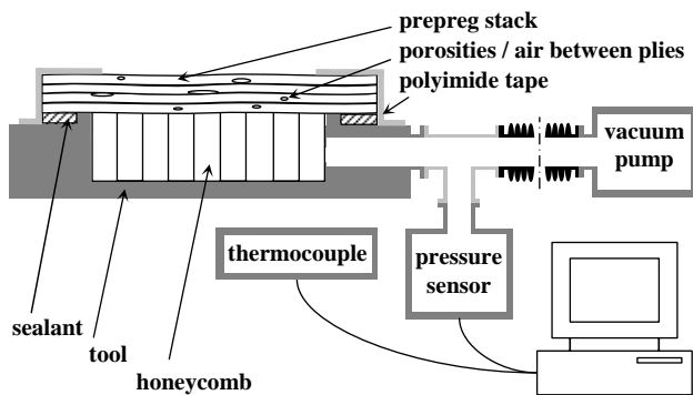
Fig. 4. Experimental set-up for measuring the intrinsic through thickness air permeability of the prepregs
