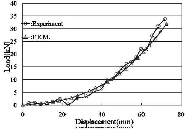
Fig.8. Comparison of experimental and predicted load-displacement curve of CFRP guarder belt for vertical impact
