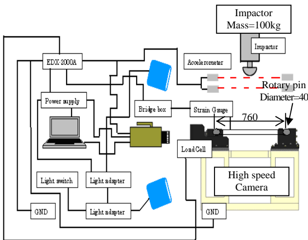
Fig.3. CFRP guarder belt specimen and Tower drop impact test setup
