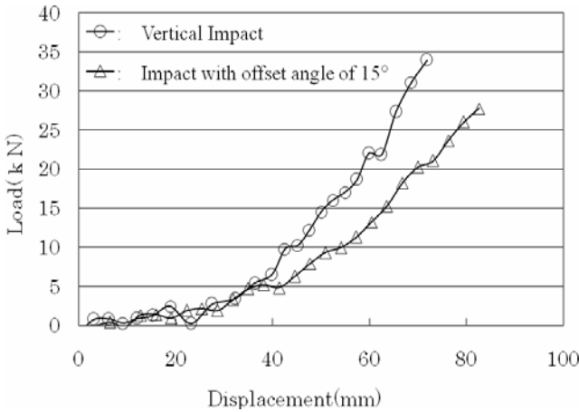
Fig.6. Comparison of experimental load-displacement curves between the vertical impact and the impact with offset angle of 15°
