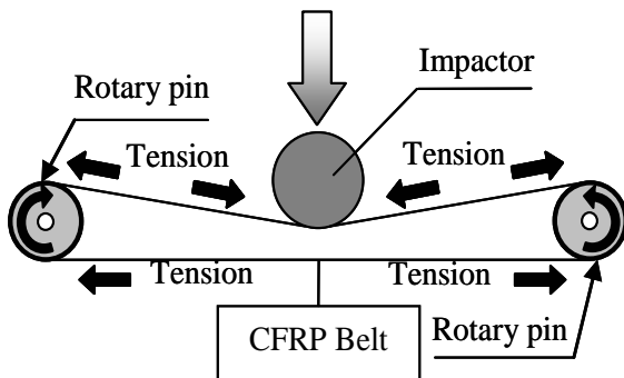
Fig.2. Energy absorption mechanism of CFRP guarder belt
