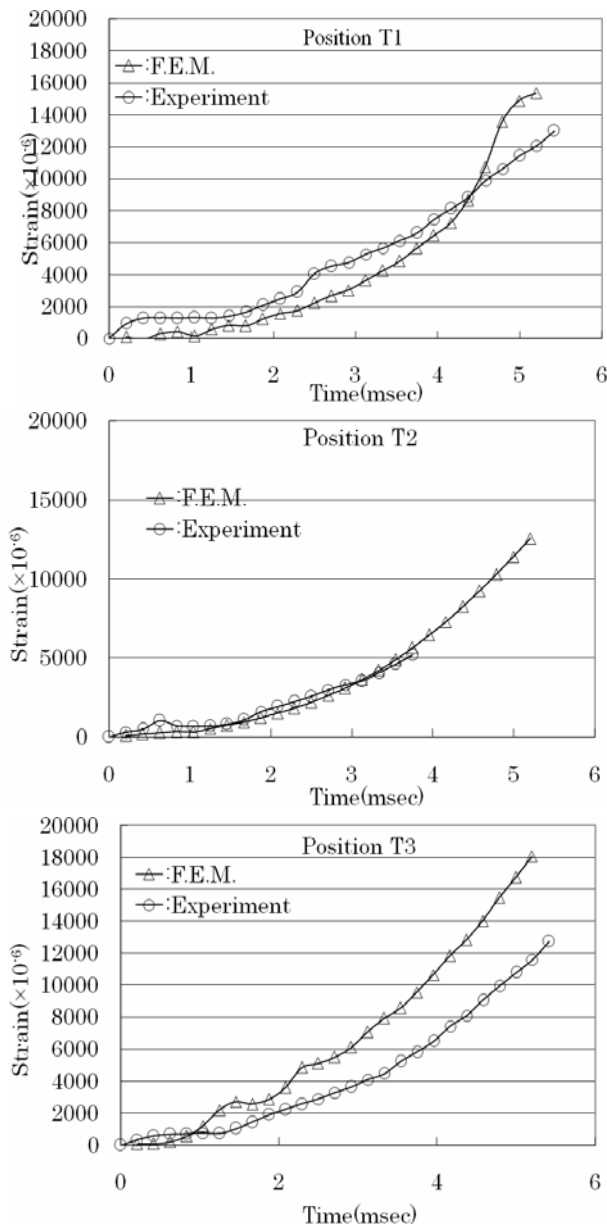
Fig.12. Comparisons of experimental and predicted the strain variation for impact with offset angle of 15 °
