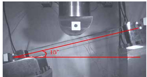
Fig.9. The drop weight impact test with offset angle of 15°
