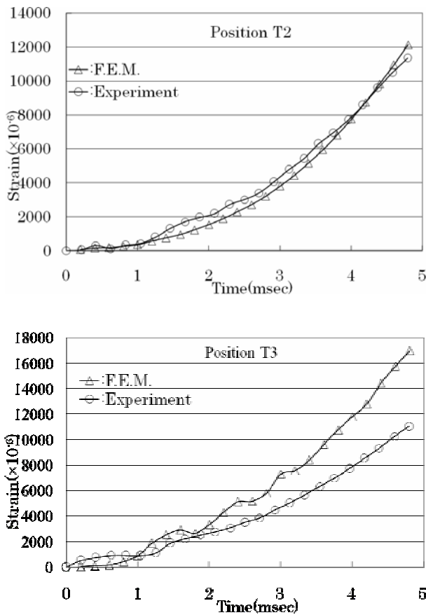
Fig.9. Comparisons of experimental and predicted the strain variation of CFRP guarder belt for vertical impact
