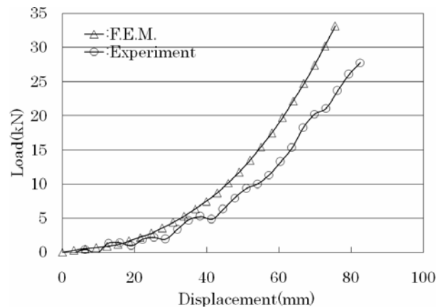
Fig.11. Comparison of experimental and predicted load-displacement curve for impact with offset angle of 15°
