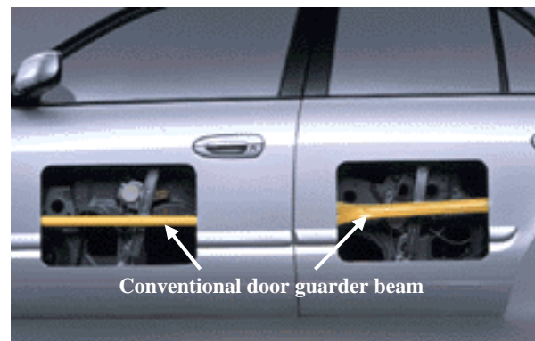
Fig.1. Conventional door guarder beam
